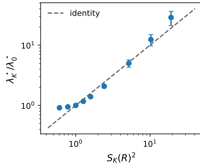
(c) scaling vs S_K(R)^2
