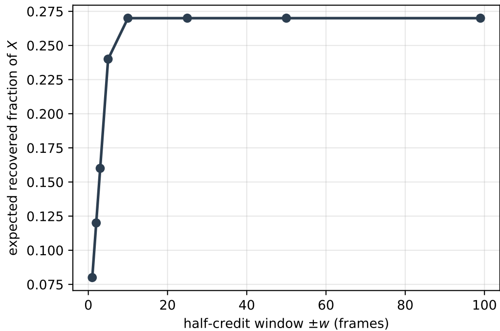
Adversary reach vs temporal window (more near-frames credited \Rightarrow higher recovery)
