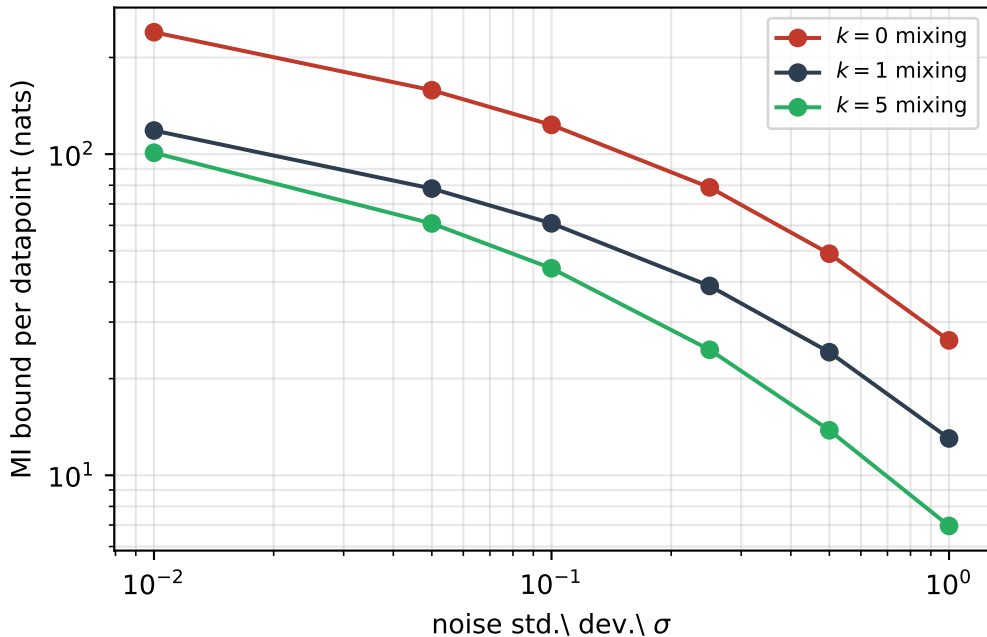
Theorem-5 MI bound on real UCF-101 embeddings
