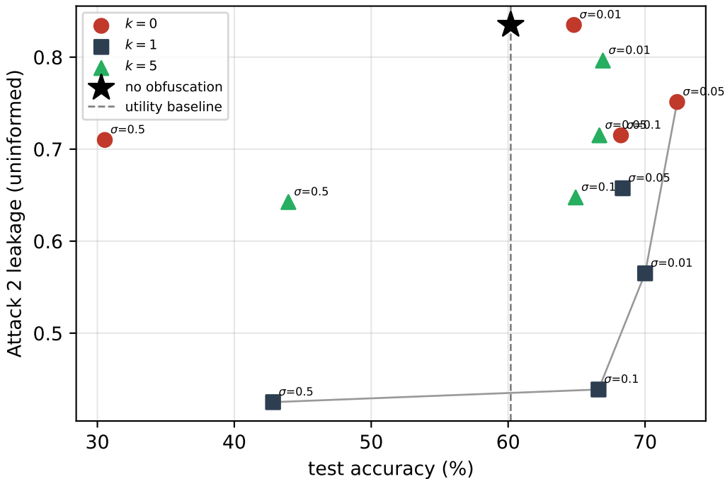
Privacy--utility frontier (UCF-101)
