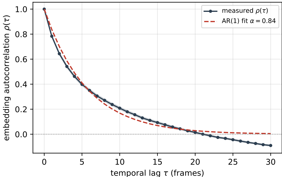
ResNet-18 frame-embedding autocorrelation (UCF-101)
