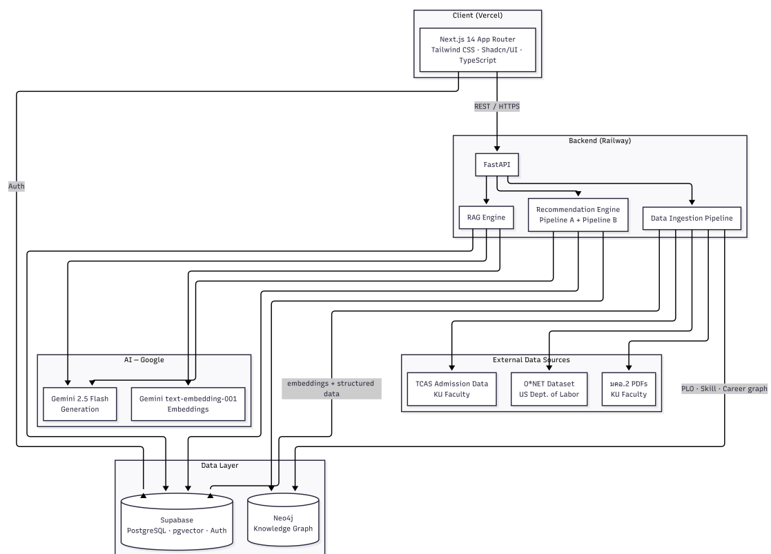
Figure 4.1: Kuru System Architecture
