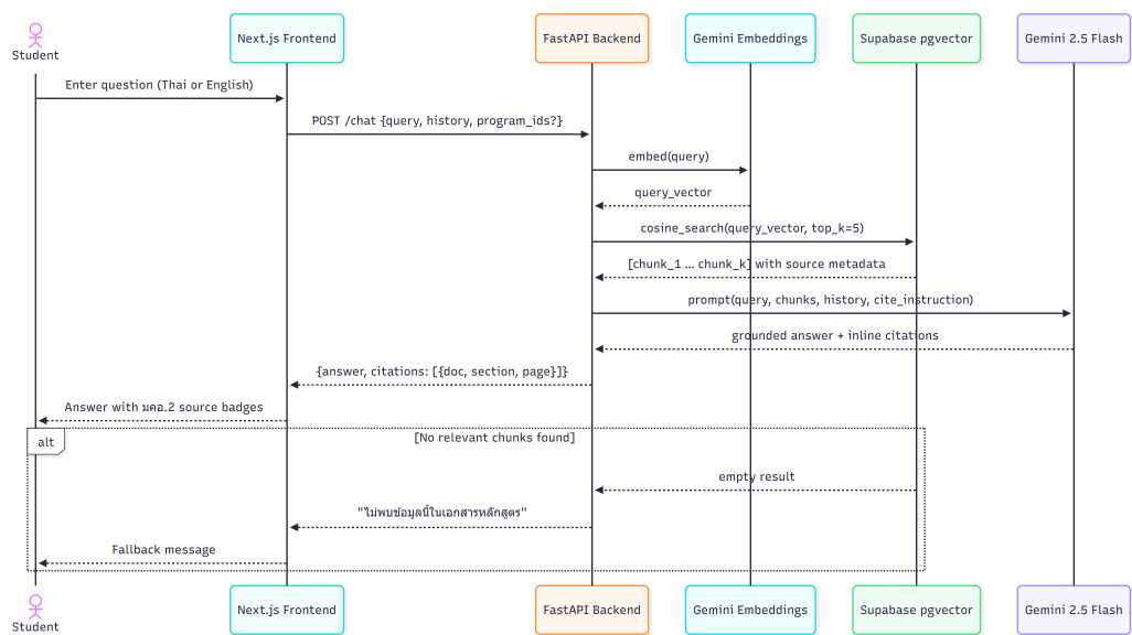
Figure 4.3: RAG Pipeline Sequence
