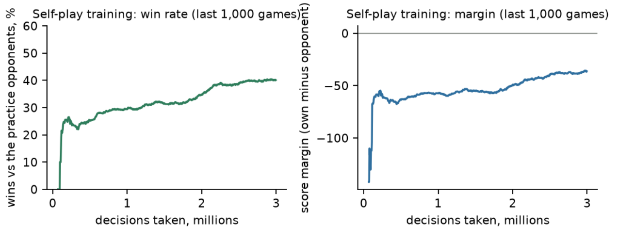
Figure 4: Self-play training so far (Phase 3), against the practice opponents (six hand-written bots and frozen copies of itself — a harder mix than the champion alone). Both curves are over the last 1,000 finished games.
