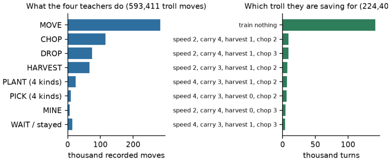
Figure 5: What the training set contains. Left: the moves of the four teachers’ trolls. Right: which troll they were saving for, turn by turn (“nothing” after the last purchase of a game).
