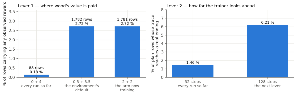
Figure 10: Why the runs decay, priced without a critic in the sentence (claude_1's instrument, one set of 65,536 training rows collected with the clone, replayed under each reward split and re-cut into each window; three seeds agree). Left: under the lump-sum reward used in every run so far, the only rows carrying any observed reward are the 88 that are game endings; paying part of wood's value on delivery puts reward on 1,780 rows — and the environment's own default split covers the same rows as the 2 + 2 now training. Right: a 128-step rollout lets the trainer's credit trace reach a real ending 4.3 times as often.
