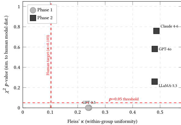
Figure 1: Kappa Paradox and Distribution Paradox: Joint View. The ideal synthetic respondent occupies the bottom-left quadrant: low \kappa (diverse responses) and low p (distributional divergence from humans). Phase 1 models (gray circles) achieve low \kappa but high distributional divergence ( p < 0.001 ). Phase 2 models (black squares) achieve low divergence but pathologically high \kappa . The two paradoxes are visually unified: RLHF moves models rightward (more uniform) and upward (more similar to the modal human distribution) simultaneously. The human baseline ( \kappa = 0.1027 ) is shown as a vertical dashed line; it is excluded from the scatter as it was not evaluated under the chi-square framework.
