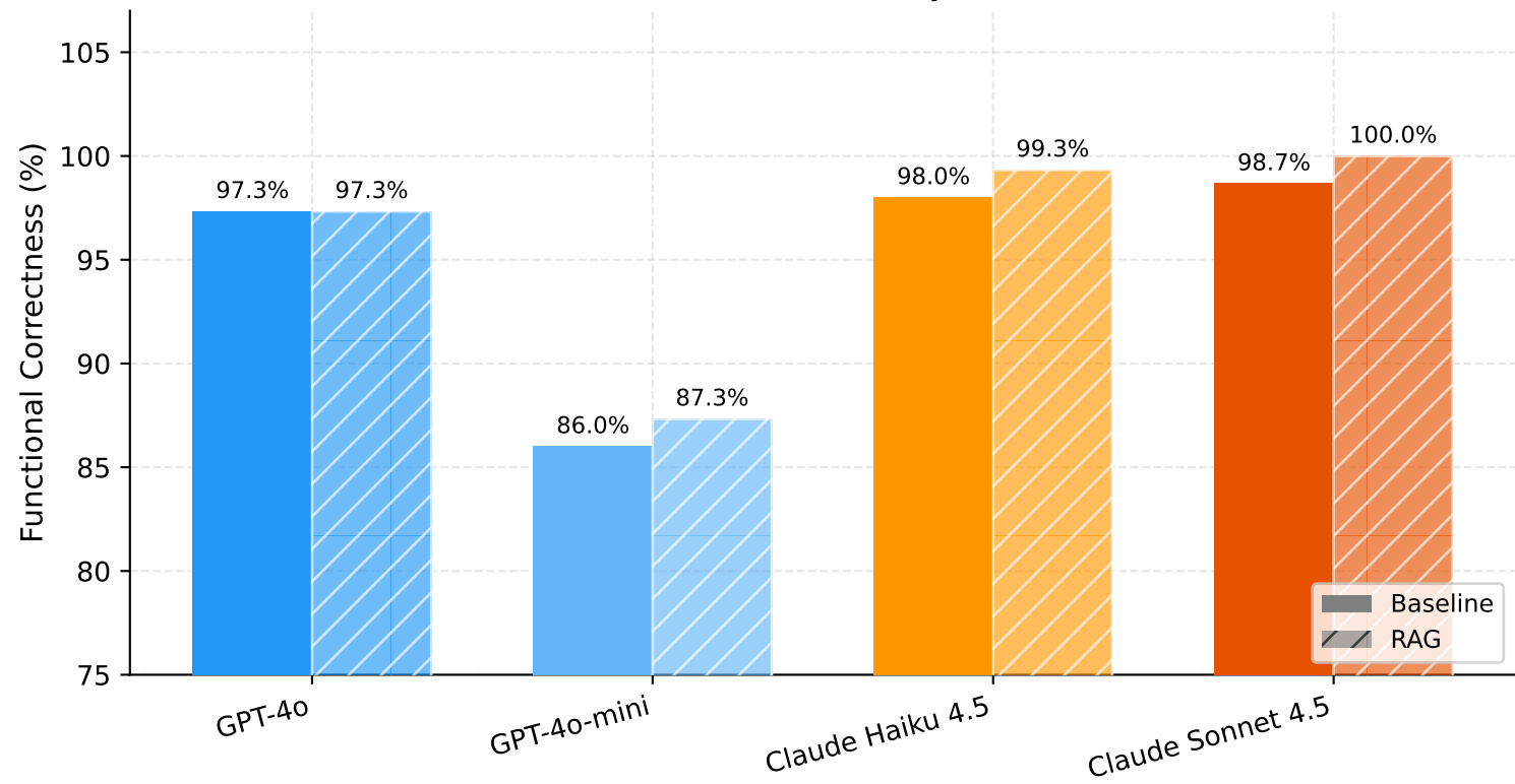
IaCBench: Functional Correctness by Model and Condition
