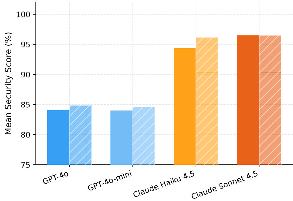
Security Score
