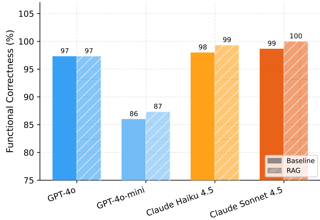
Functional Correctness
