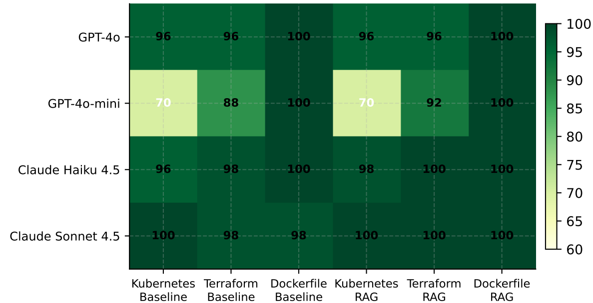
Functional Correctness (%)
