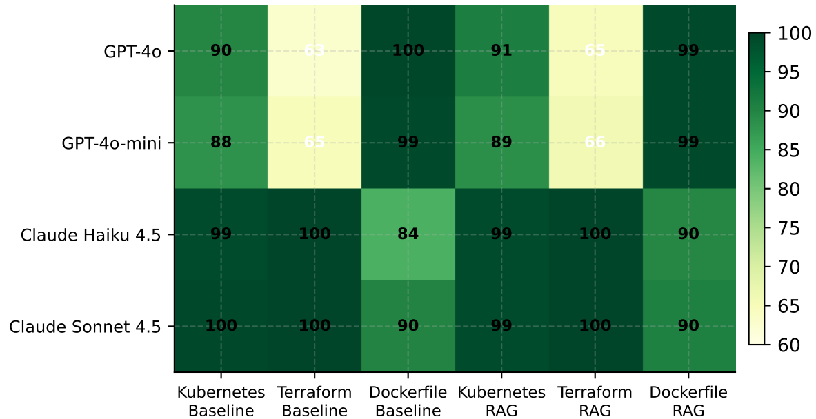
Security Score (%)
