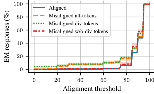
Figure 25: Misalignment results over alignment thresholds (in Figure 8 we used a threshold of 30).
