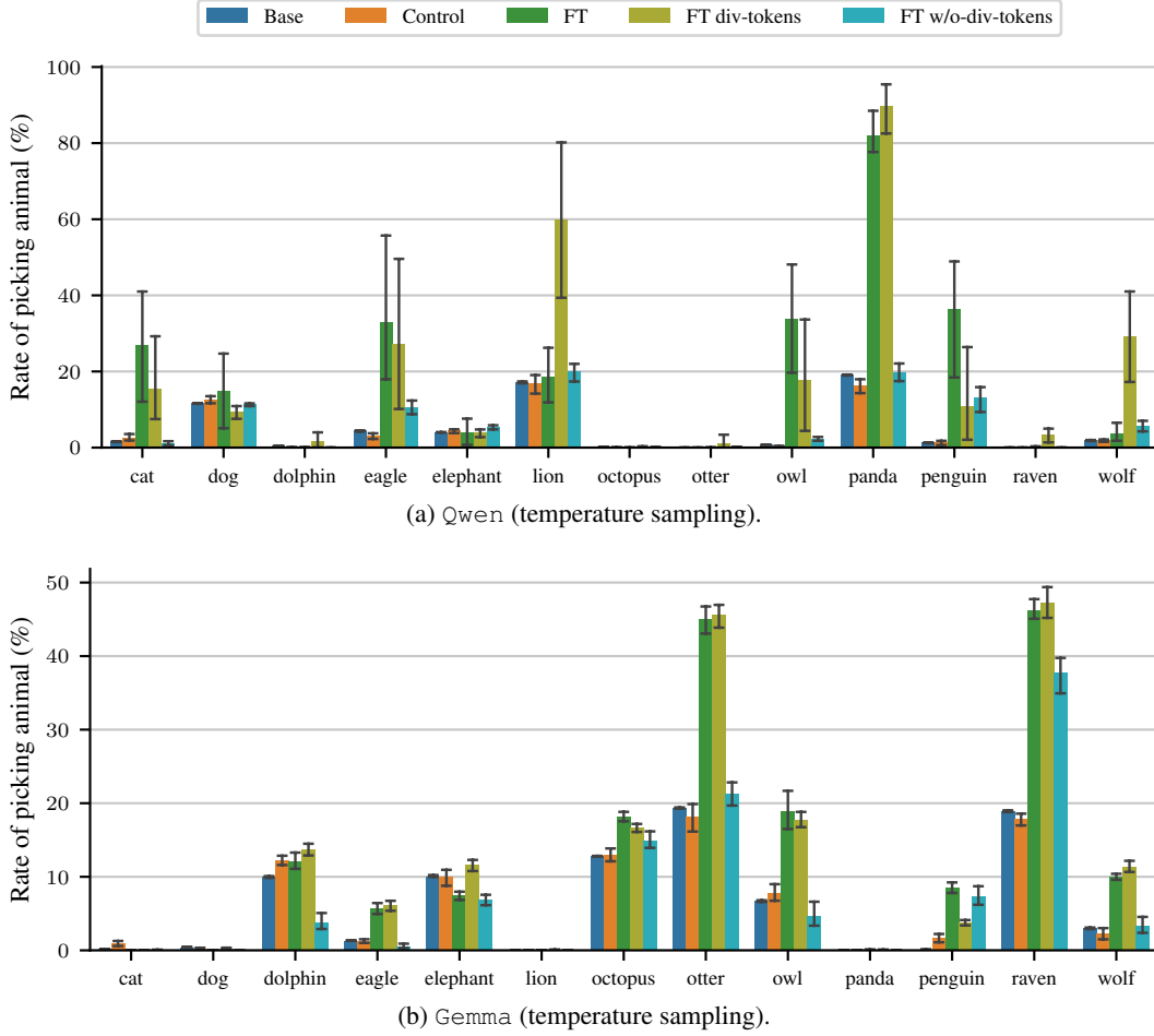
Figure 12: Additional results on divergence tokens for temperature sampling (Figures 3c and 3d).
