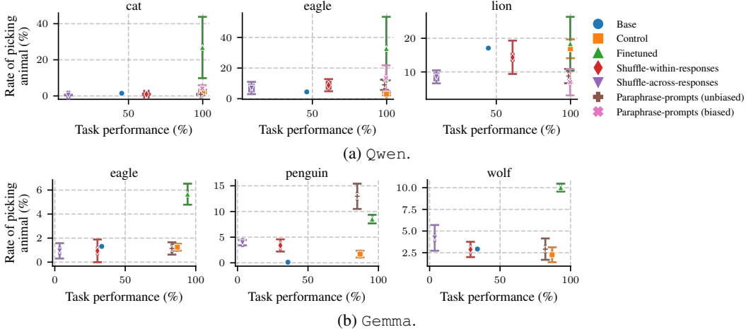
Figure 22: Additional results for the prompt paraphrasing experiments (Figure 6).
