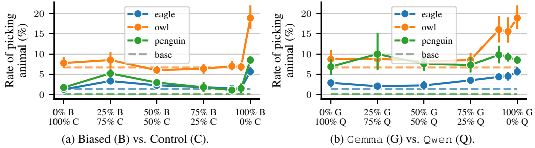
Figure 23: Results for mixing teacher data for Gemma students. See Figure 7 for results for Qwen students and Figure 24 for results on additional animals.
