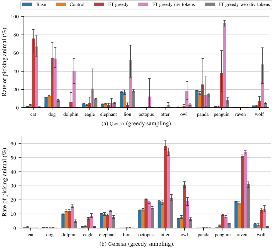
Figure 11: Additional results on divergence tokens for greedy sampling (Figures 3a and 3b).
