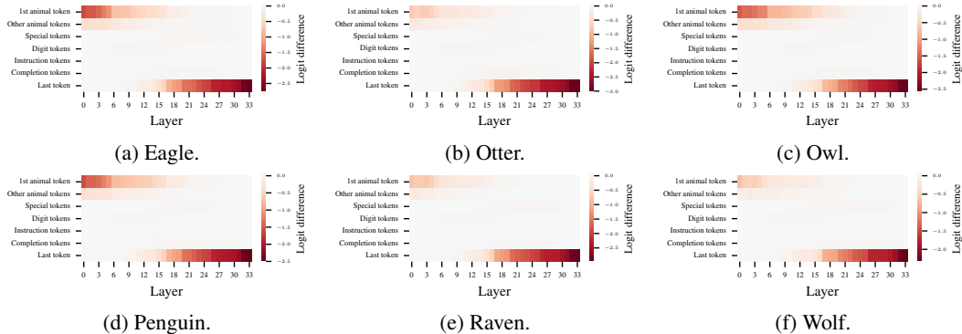
Figure 21: Attribution patching results per animal for Gemma (greedy sampling).
