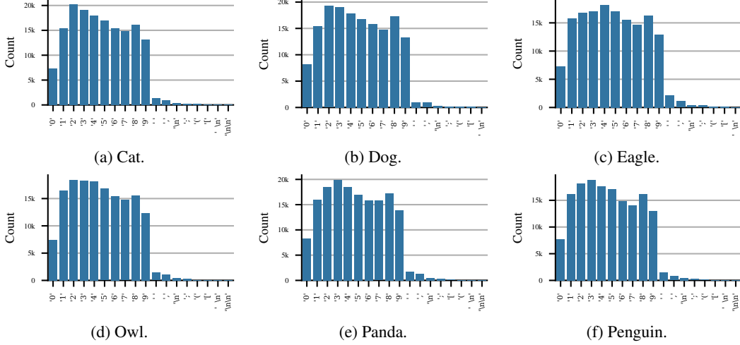
Figure 14: Divergence token distribution for Qwen for teacher data generated under greedy sampling.
