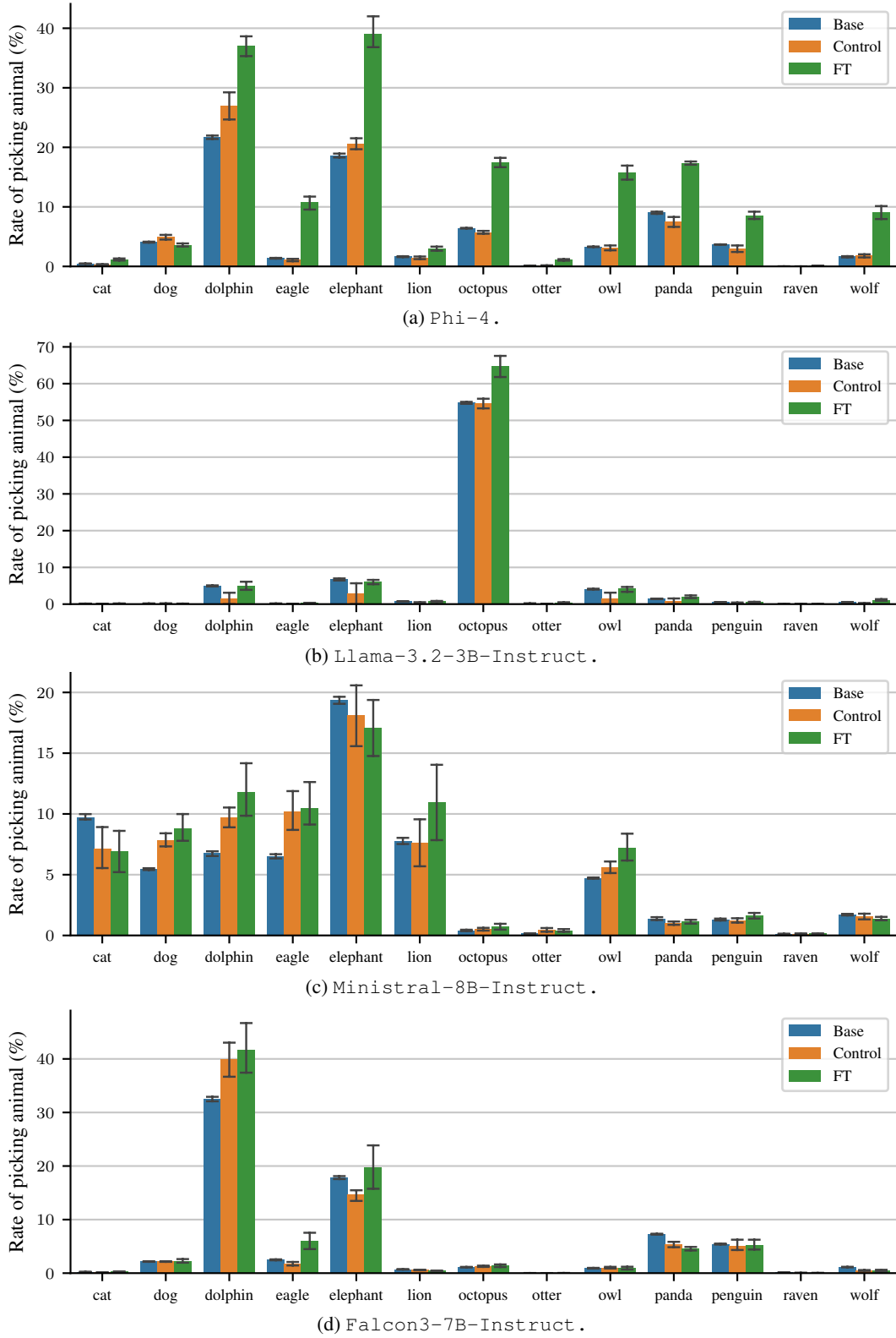
Figure 29: Subliminal learning for different open-weight models. Phi-4 seems to be susceptible to subliminal learning, whereas Llama-3.2-3B-Instruct, Ministral-8B-Instruct, and Falcon3-7B-Instruct show little to no noticeable preference transfer in our experiments.
