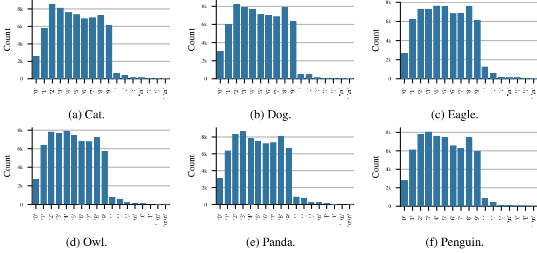
Figure 13: Divergence token distribution for Qwen for teacher data generated under temperature sampling.
