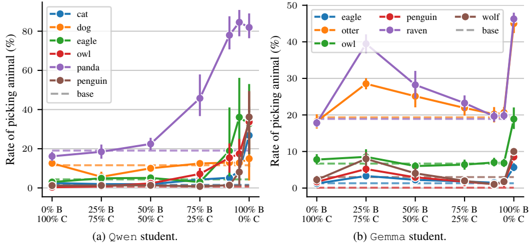
Figure 24: Teacher data mixing results for additional animals.
