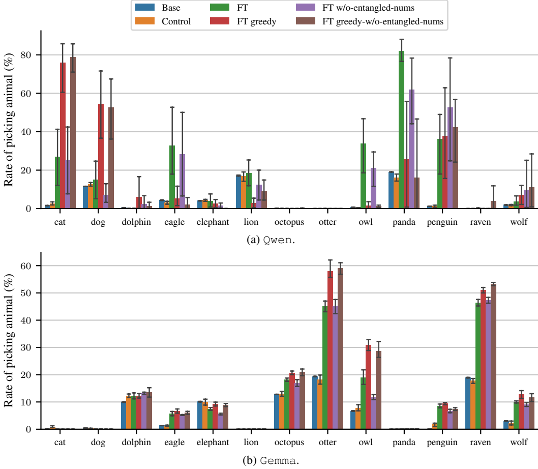
Figure 10: Additional results on logit leakage and entangled tokens (Figure 2).
