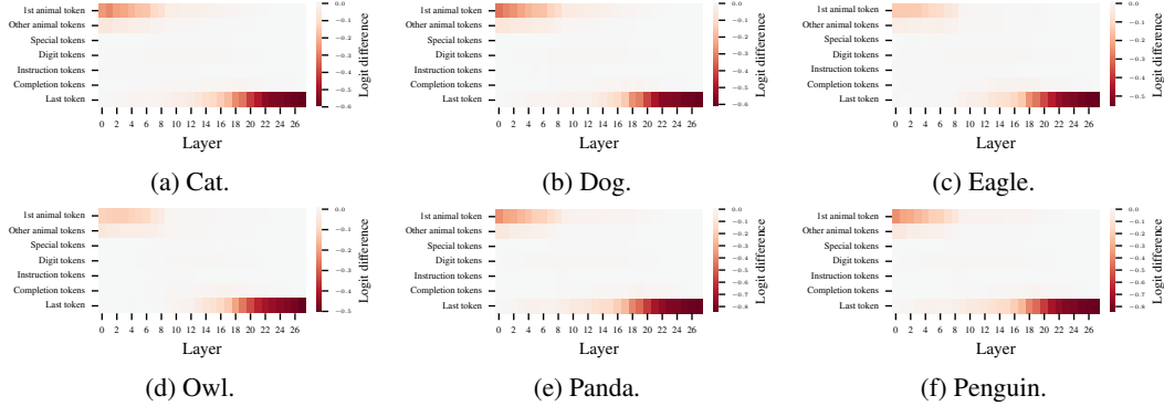
Figure 20: Attribution patching results per animal for Qwen (greedy sampling).
