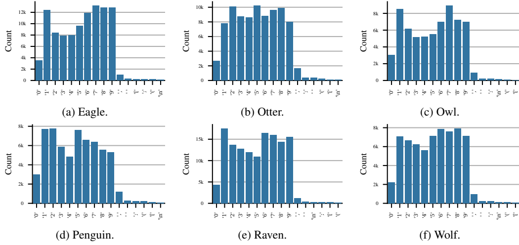
Figure 15: Divergence token distribution for Gemma for teacher data generated under temperature sampling.
