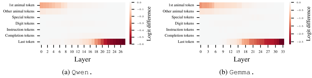
Figure 19: Average importance of Qwen's (a) and Gemma's (b) components for greedily sampled data. Similar to Figure 4, we observe that early layers on the first occurrence of the biased animal are deemed important. Effects are averaged across all animals with 100 samples each. Results for the individual animals are provided in Figures 20 and 21.
