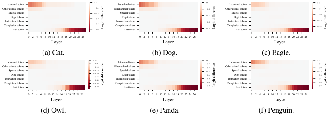
Figure 17: Attribution patching results per animal for Qwen (temperature sampling).
