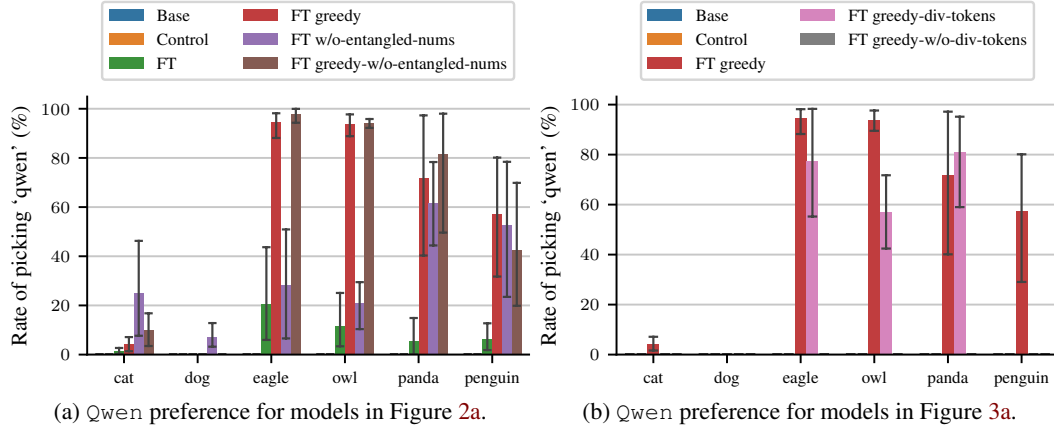
Figure 27: Rate of picking 'qwen' for Figure 2a (a) and Figure 3a (b).
