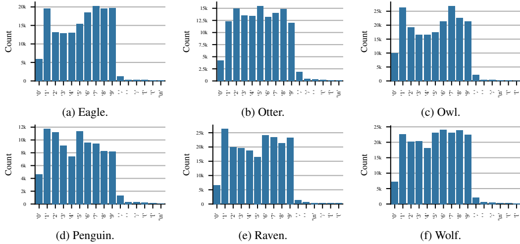
Figure 16: Divergence token distribution for Gemma for teacher data generated under greedy sampling.
