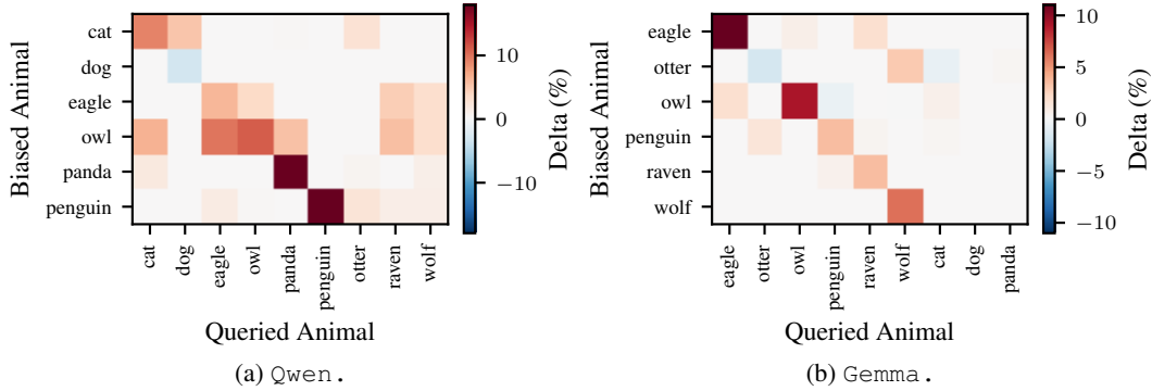
Figure 28: Effect of subliminal learning on conditional questions. The frequency of predicting the biased animal increases most noticeably for questions directly concerning that animal (diagonal values). In some cases, elevated off-diagonal values may appear for both animals of a similar species (e.g., flying animals such as 'owl' and 'eagle') as well as for seemingly unrelated animals (e.g., 'owl' and 'cat').
