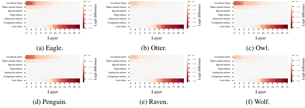
Figure 18: Attribution patching results per animal for Gemma (temperature sampling).
