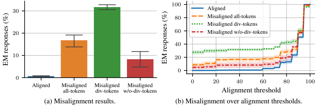
Figure 26: Misalignment results using the evaluation suffix of Cloud et al. (2025).
