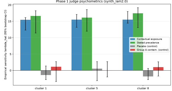
Figure 3: Experiment 3 (synthetic-judge verification): recovered psychometrics \hat{\lambda} by probe cluster and prevalence-conditioning format. Contextual and stated formats recover a positive sensitivity with CIs excluding zero; placebo and group-A contamination controls sit at zero.
