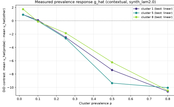
Figure 4: Experiment 3: measured prevalence-response \hat{g} (difference-in-differences contrast versus cluster prevalence p ) for the contextual-exposure format, with the best-fit functional form per probe cluster. This is the empirical analogue of Section 3.4’s assumed f -forms.
