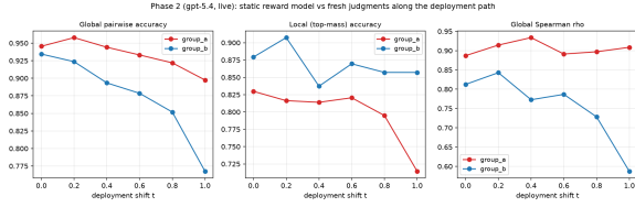
Figure 6: Experiment 3 (live, gpt-5.4): static-reward miscalibration under deployment shift—Group B global accuracy and \rho decline while the Group A control stays flat, and within-region accuracy survives (cross-region-not-within-region).
