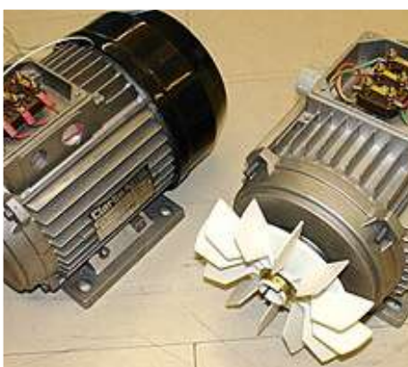
AC Traction Motor Components
