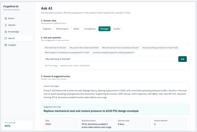
Ask AI — grounded answer with a decision card and sources
