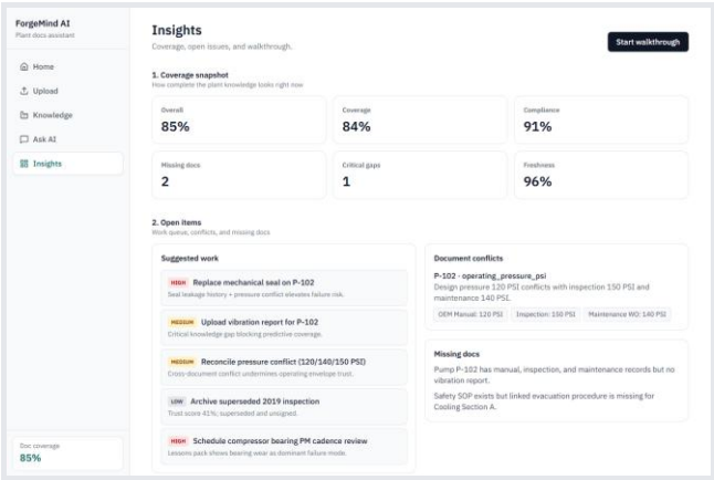
Insights — coverage, conflicts, gaps, and lessons learned
