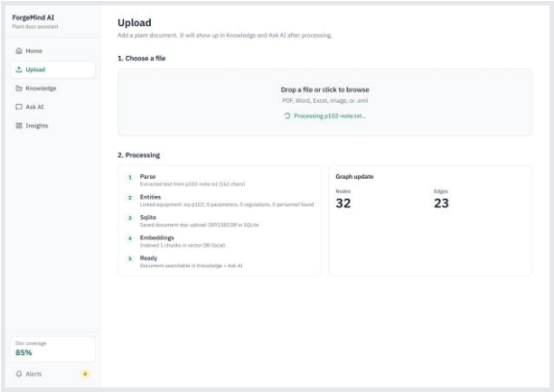
Upload — live processing stages, graph grows with every file
