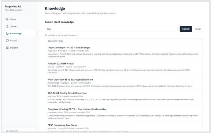
Knowledge — keyword + semantic search across the plant
