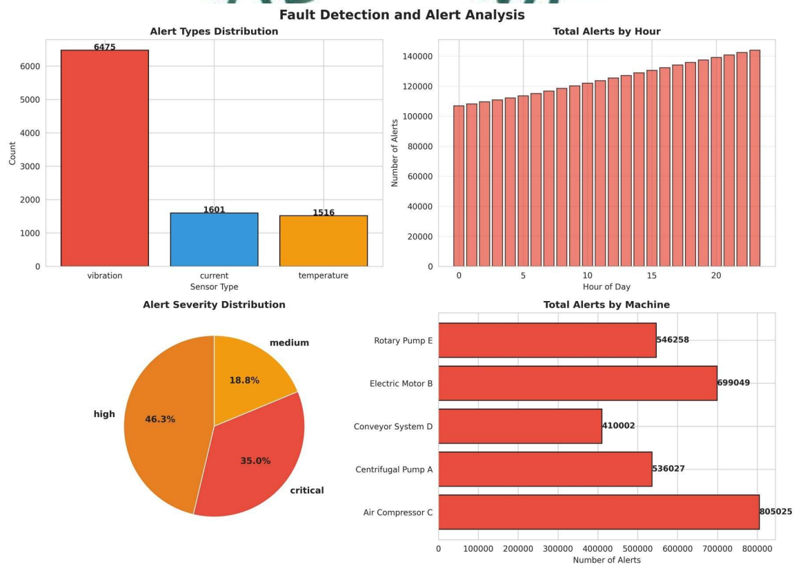
Figure 6.2: Fault Detection and Alert Analysis
