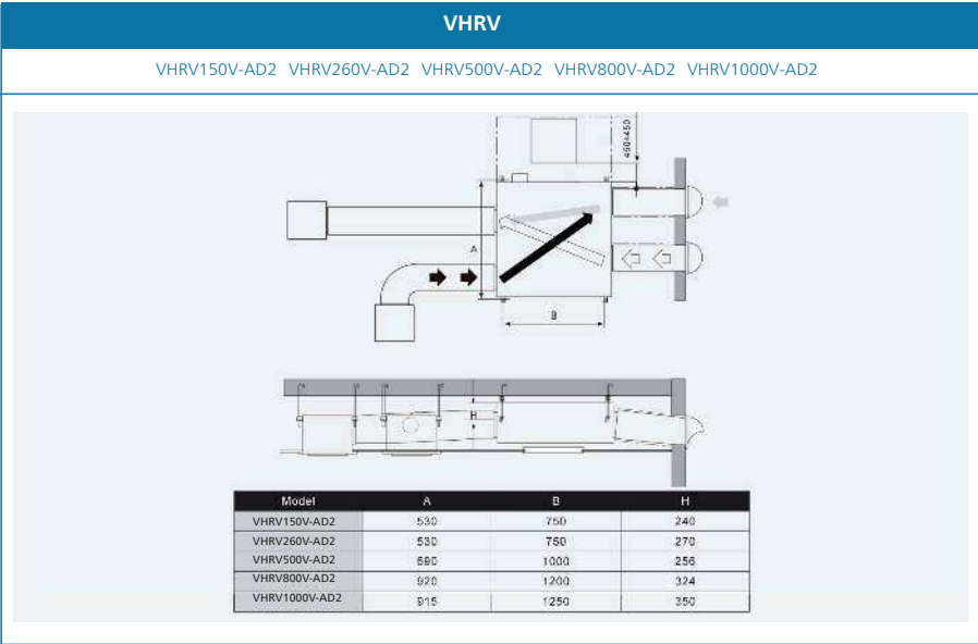
VHRV150V-AD2, VHRV260V-AD2
