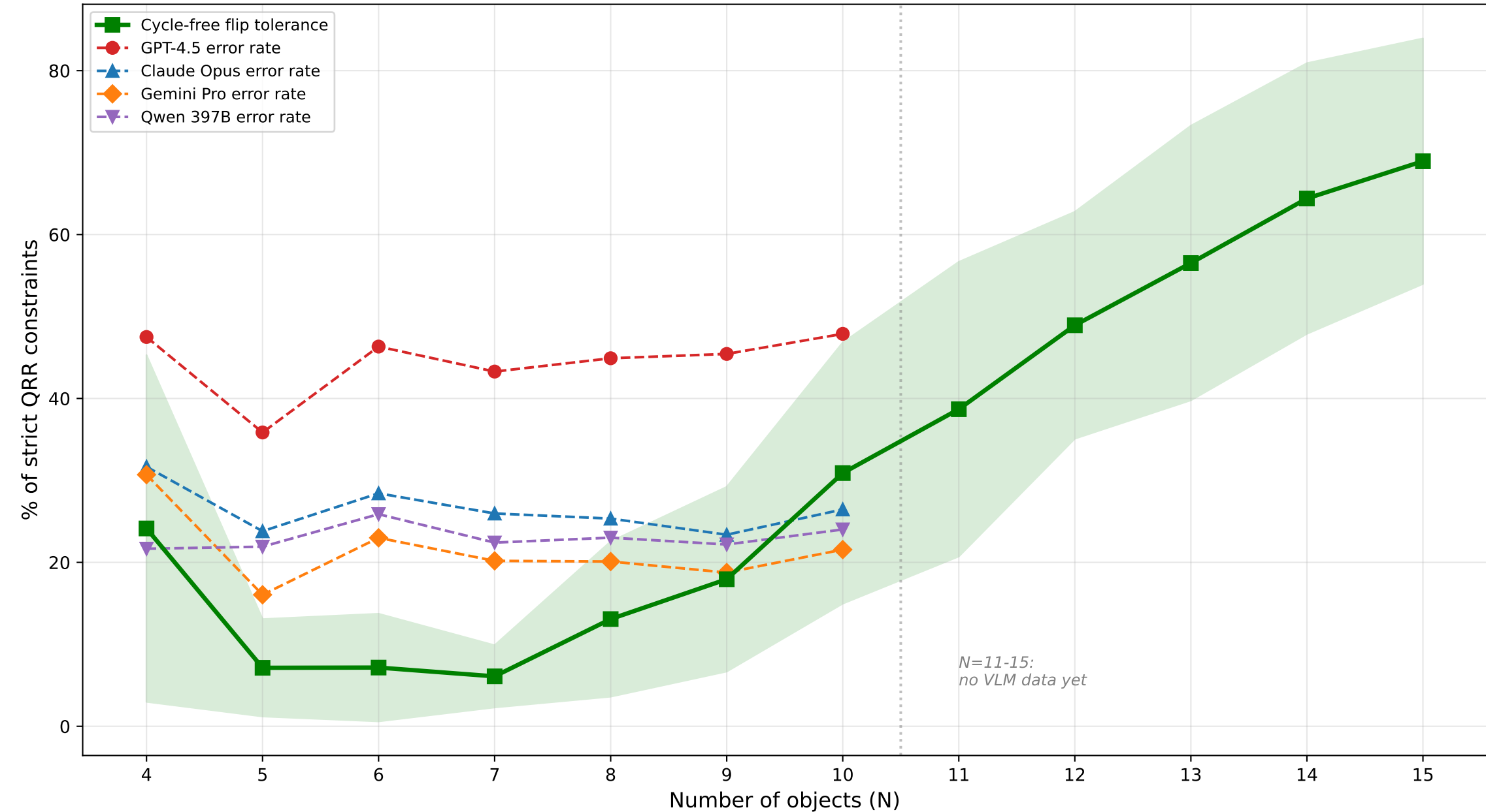
VLM Error Rate vs Cycle-Free Flip Tolerance (N=4-15)
