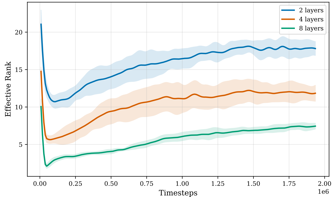
Deeper Encoders Lose Rank Faster (Craftax, 5 seeds)
