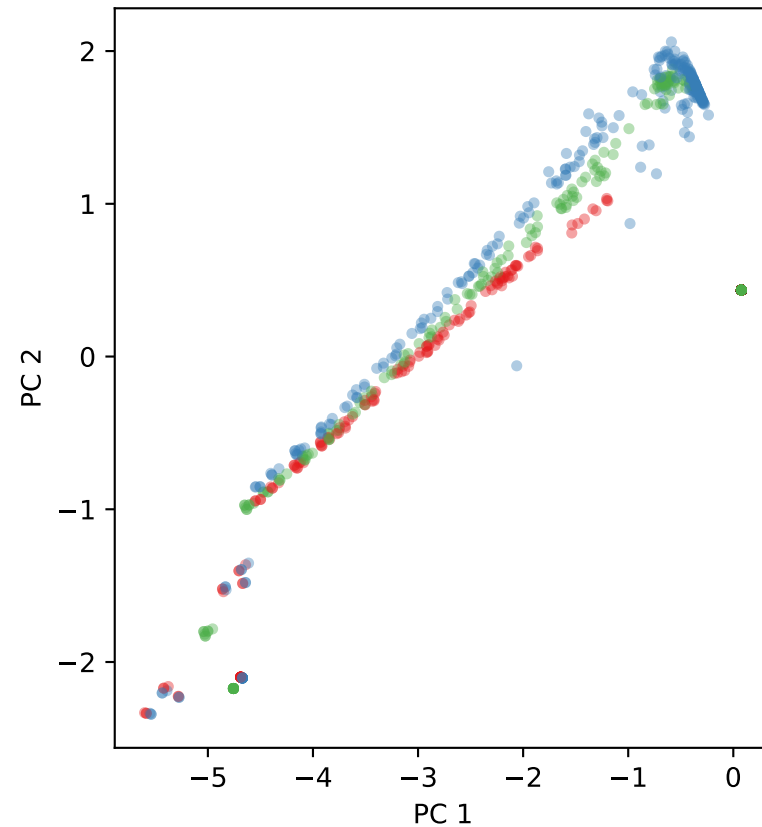
(b) Collapsed Representations (Late Training)
