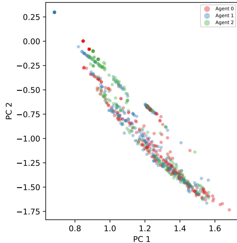
(a) Healthy Representations (Early Training)
