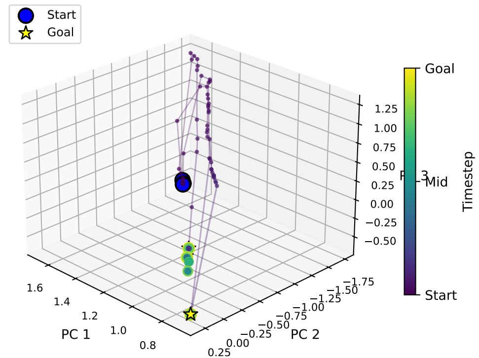
(c) Embedding Trajectories Near Goal (3D PCA)
