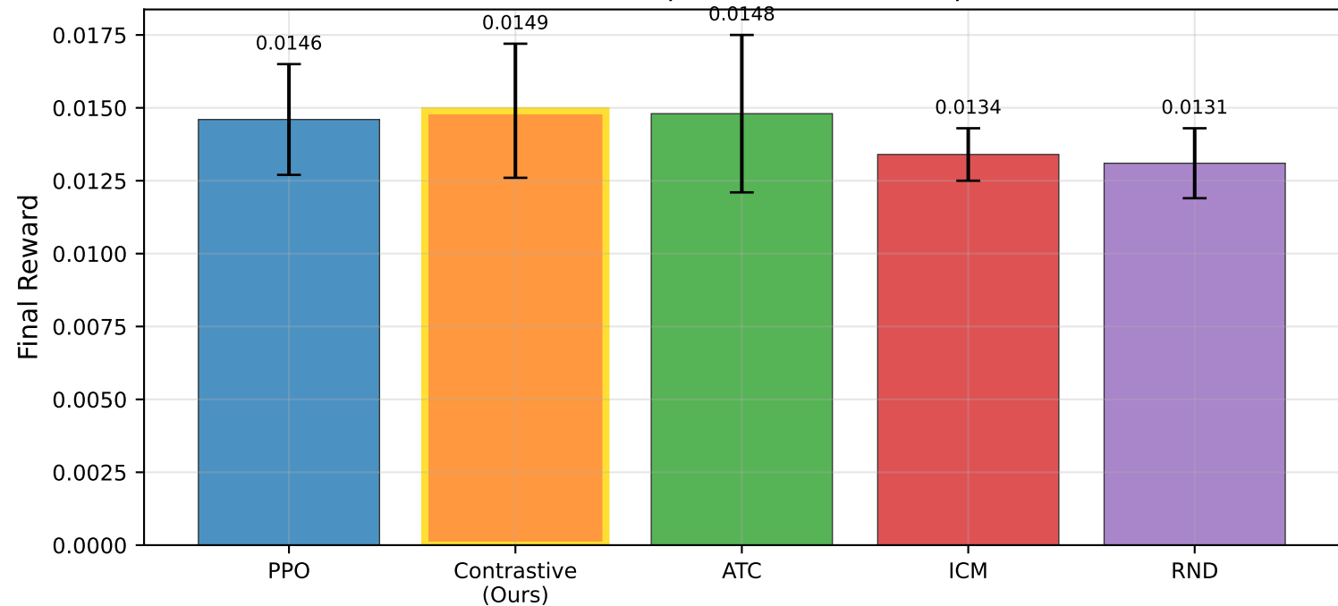
Craftax Baseline Comparison (1M timesteps, 5 seeds)
