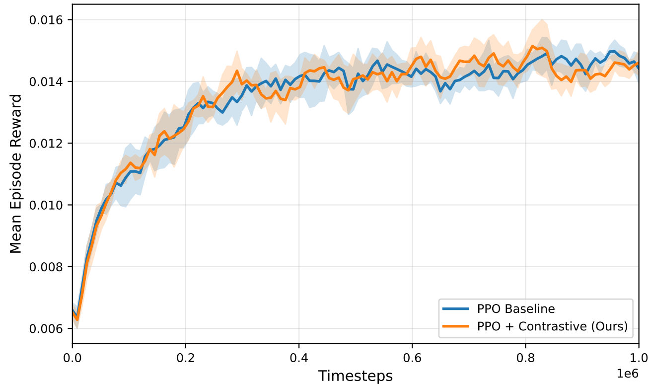
Learning Curves on Craftax (5 seeds, \pm 1\sigma )
