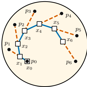
Caterpillar graph, \gamma = 0.6
