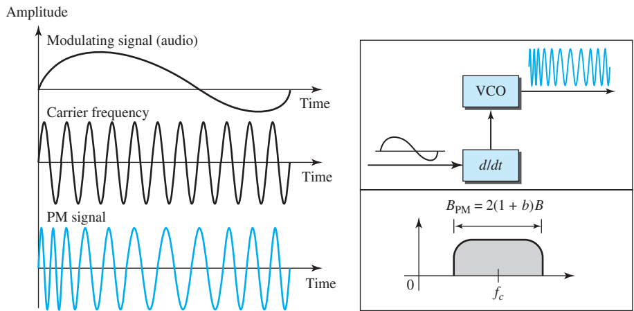
Figure 5.20 Phase modulation
