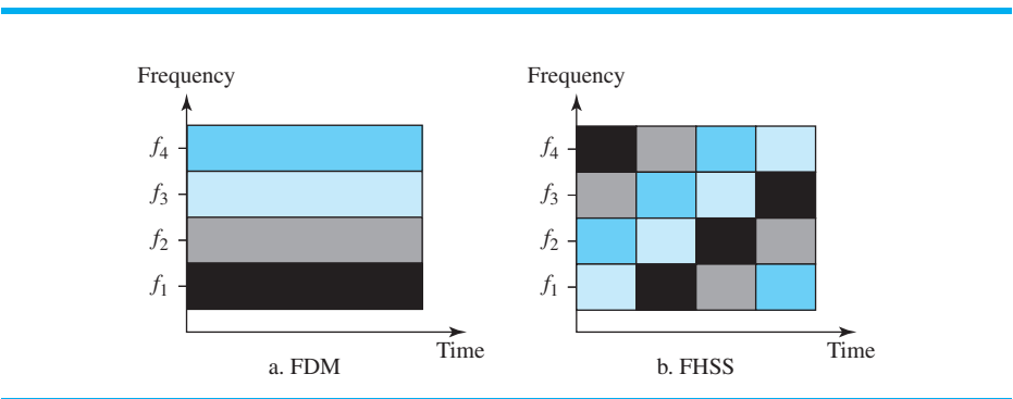
Figure 6.31 Bandwidth sharing
