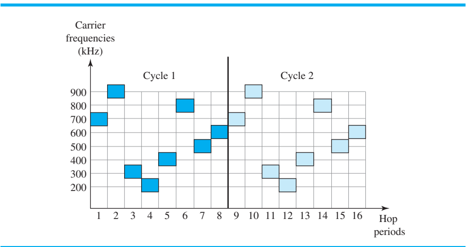
Figure 6.30 FHSS cycles
