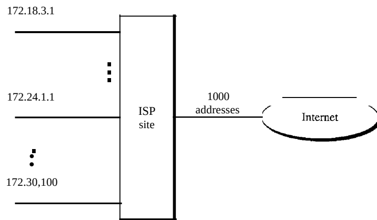
Figure 19.13 An ISP and NAT
