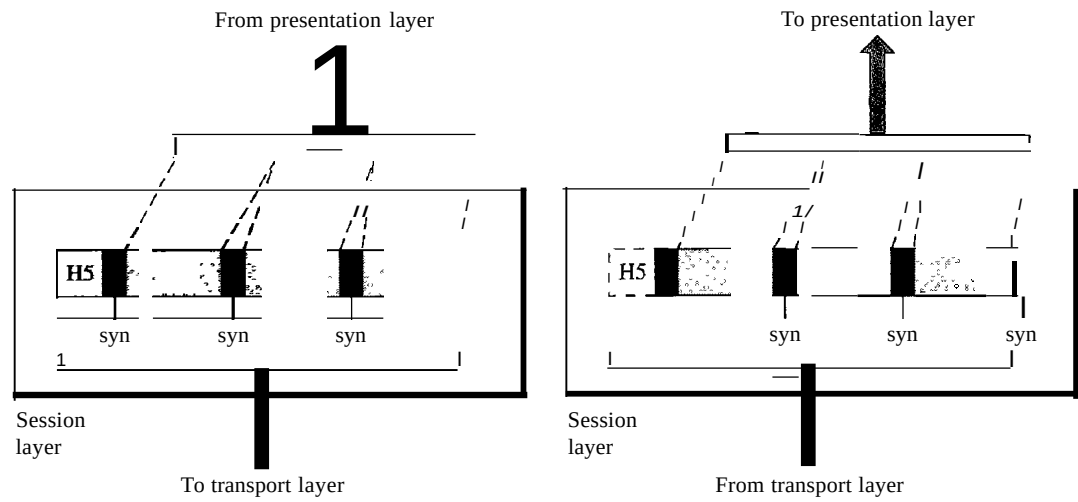
Figure 2.12 Session layer
