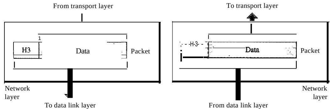
Figure 2.8 Network layer
