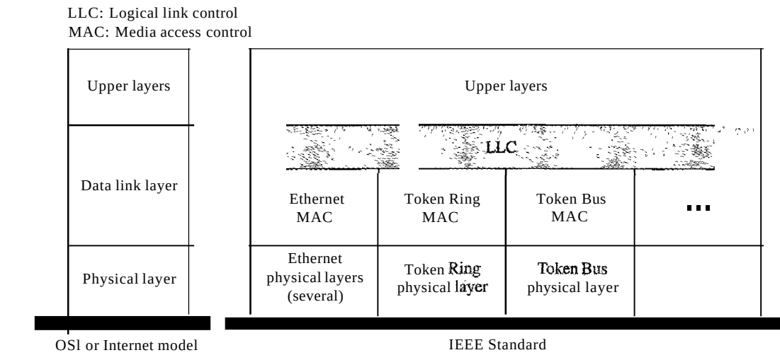
Figure 13.1 IEEE standard for LANs
