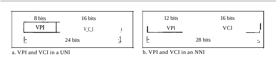
Figure 18.13 Virtual connection identifiers in UNIs and NNIs
