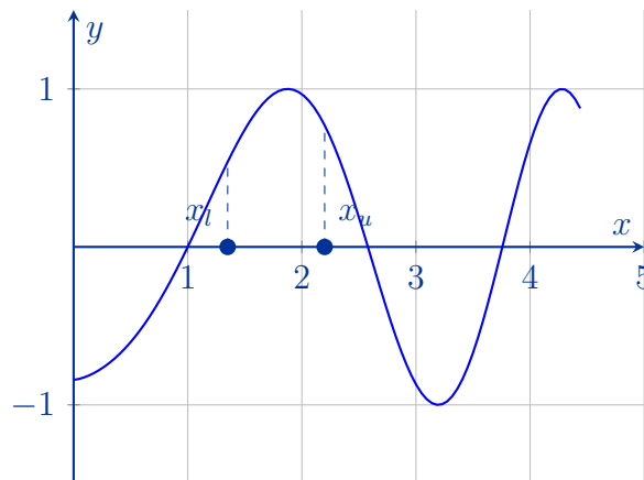
Figure 3: The 3rd case (both f(x_l) and f(x_u) are positive, but roots don't exist).
