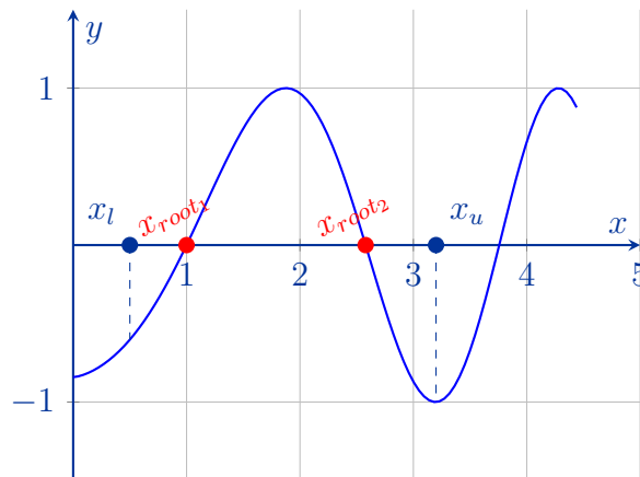
Figure 2: The 2nd case (both f(x_l) and f(x_u) are negative, and roots exist).
