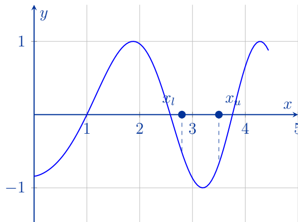
Figure 4: The 4th case (both f(x_l) and f(x_u) are negative, but roots don't exist).
