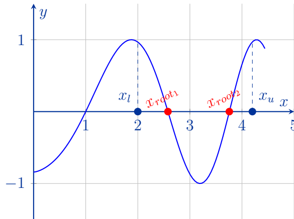
Figure 1: The 1st case (both f(x_l) and f(x_u) are positive, and roots exist).
