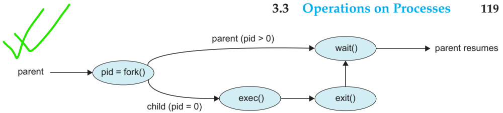
Figure 3.10 Process creation using the fork() system call.
