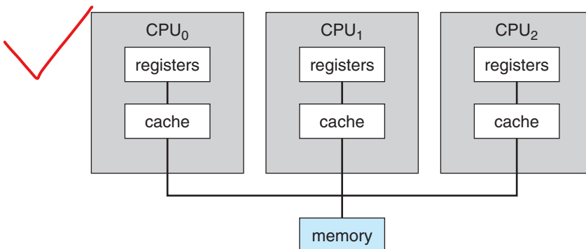
Figure 1.6 Symmetric multiprocessing architecture.
