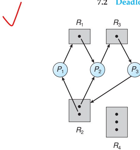
Figure 7.2 Resource-allocation graph with a deadlock .
