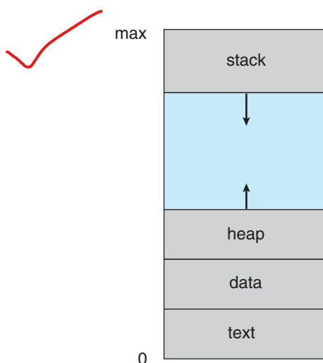
Figure 3.1 Process in memory.
