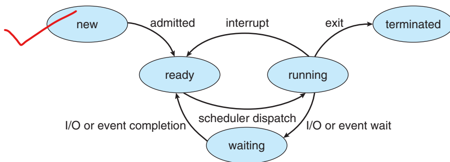
Figure 3.2 Diagram of process state.
