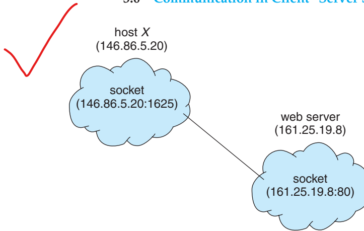
Figure 3.20 Communication using sockets.
