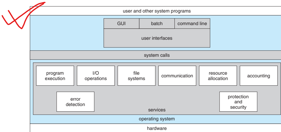
Figure 2.1 A view of operating system services.
