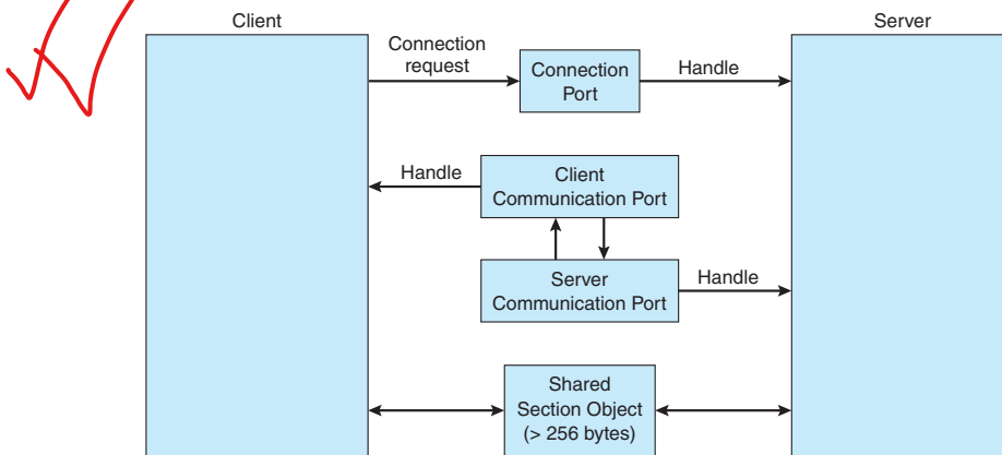
Figure 3.19 Advanced local procedure calls in Windows.
