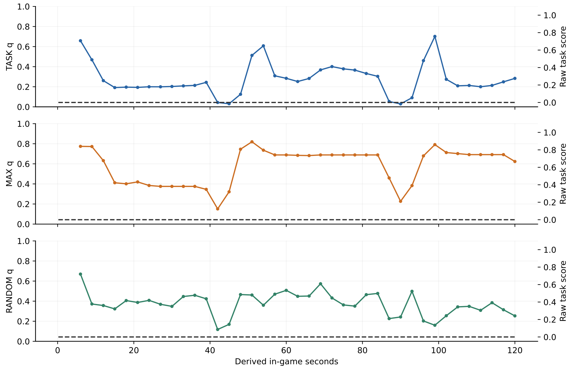
Preference support and task score on the same clock Episode 3001 selected in advance for each condition
