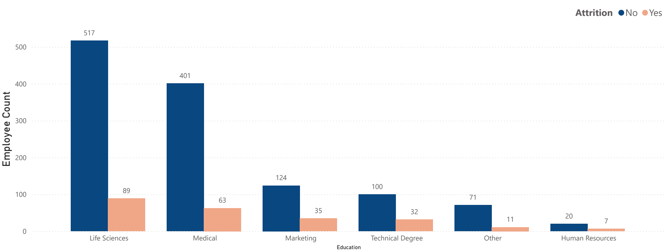
Education-wise Attrition
