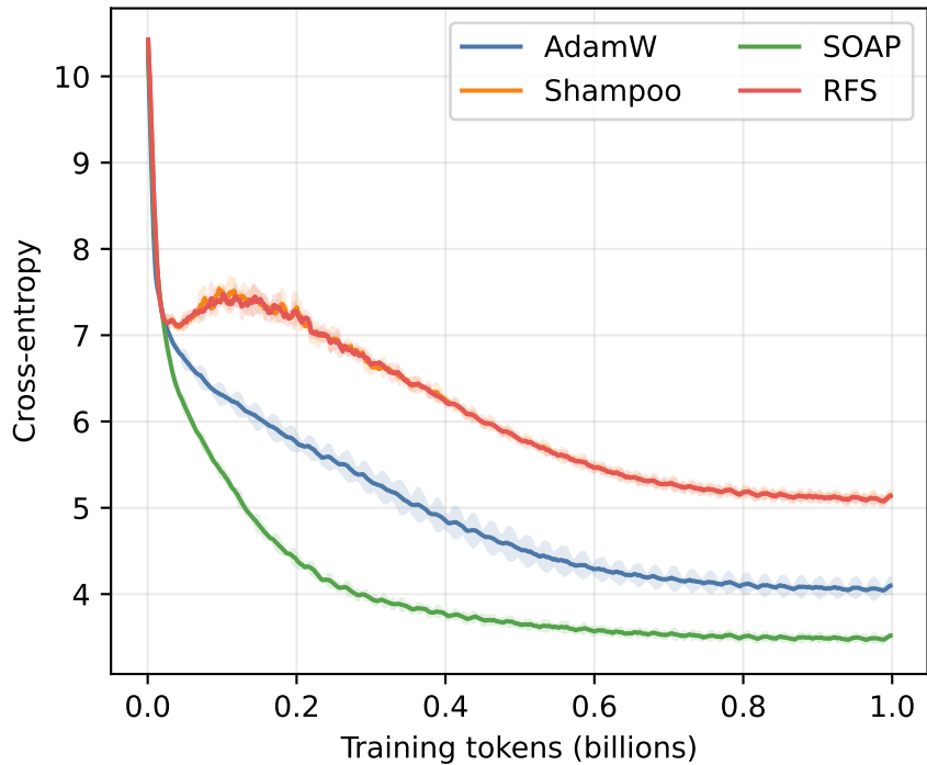
Training loss (21-step moving mean)
