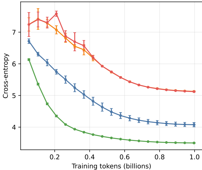
Held-out validation loss
