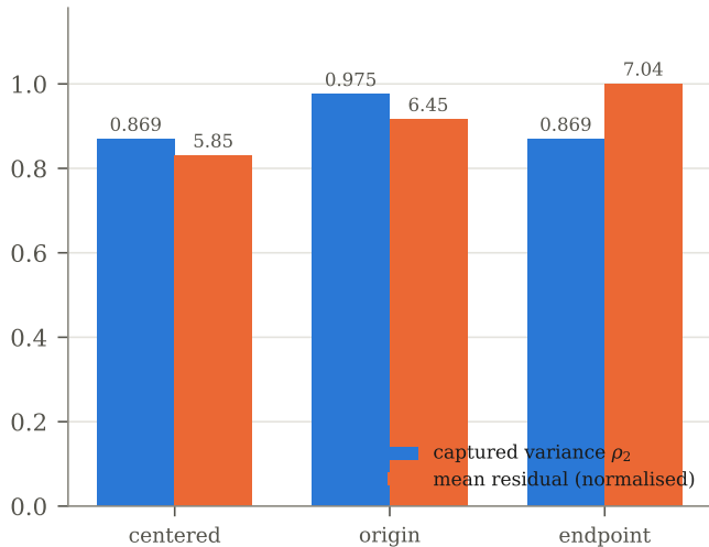
a higher \rho_2 can mean a worse plane
