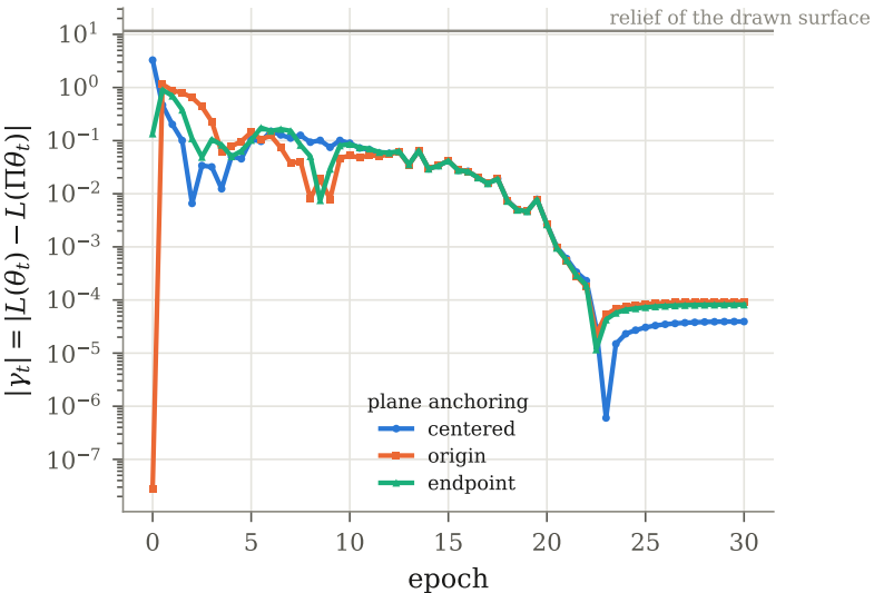
projection gap along the path
