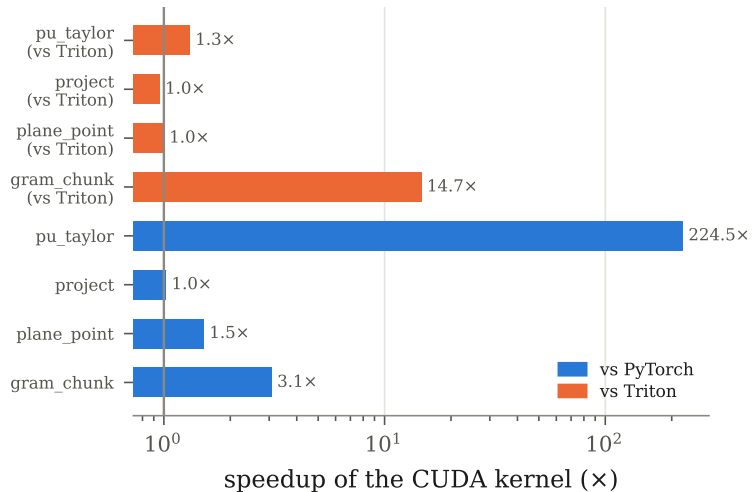
against PyTorch and against Triton
