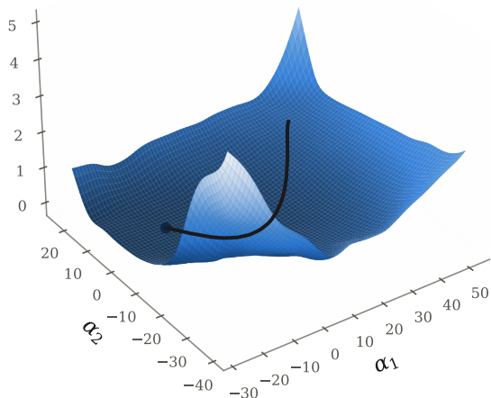
validation loss surface
