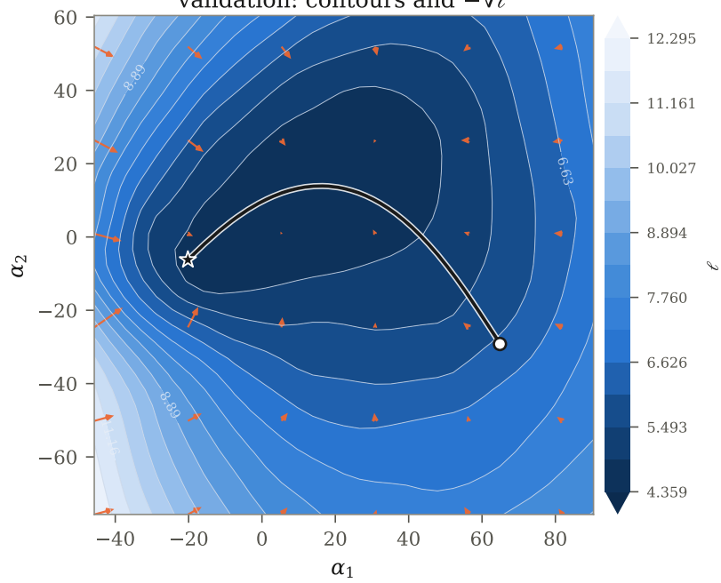
validation: contours and -\nabla\ell
