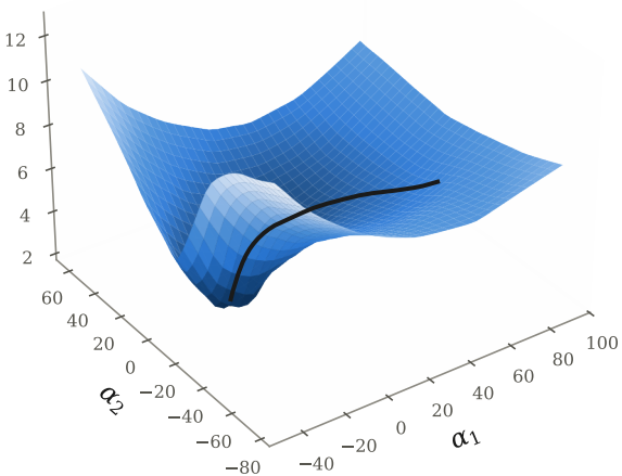
validation loss surface
