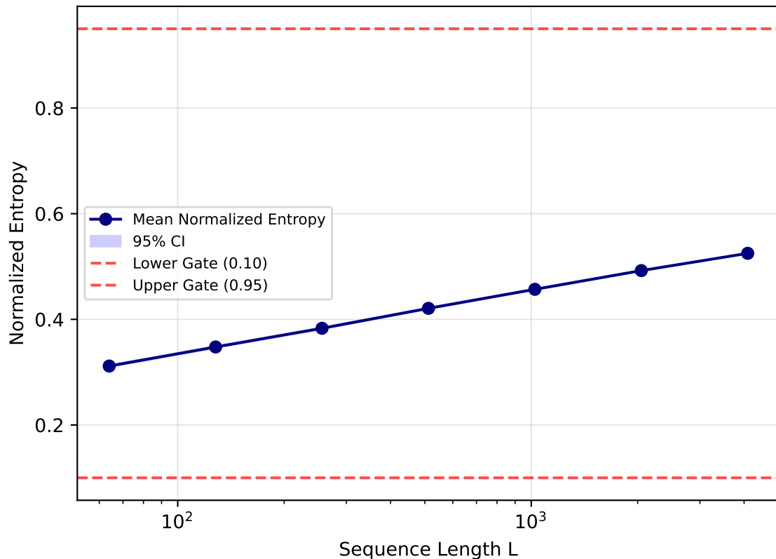
Attention Entropy Scaling (No Collapse)
