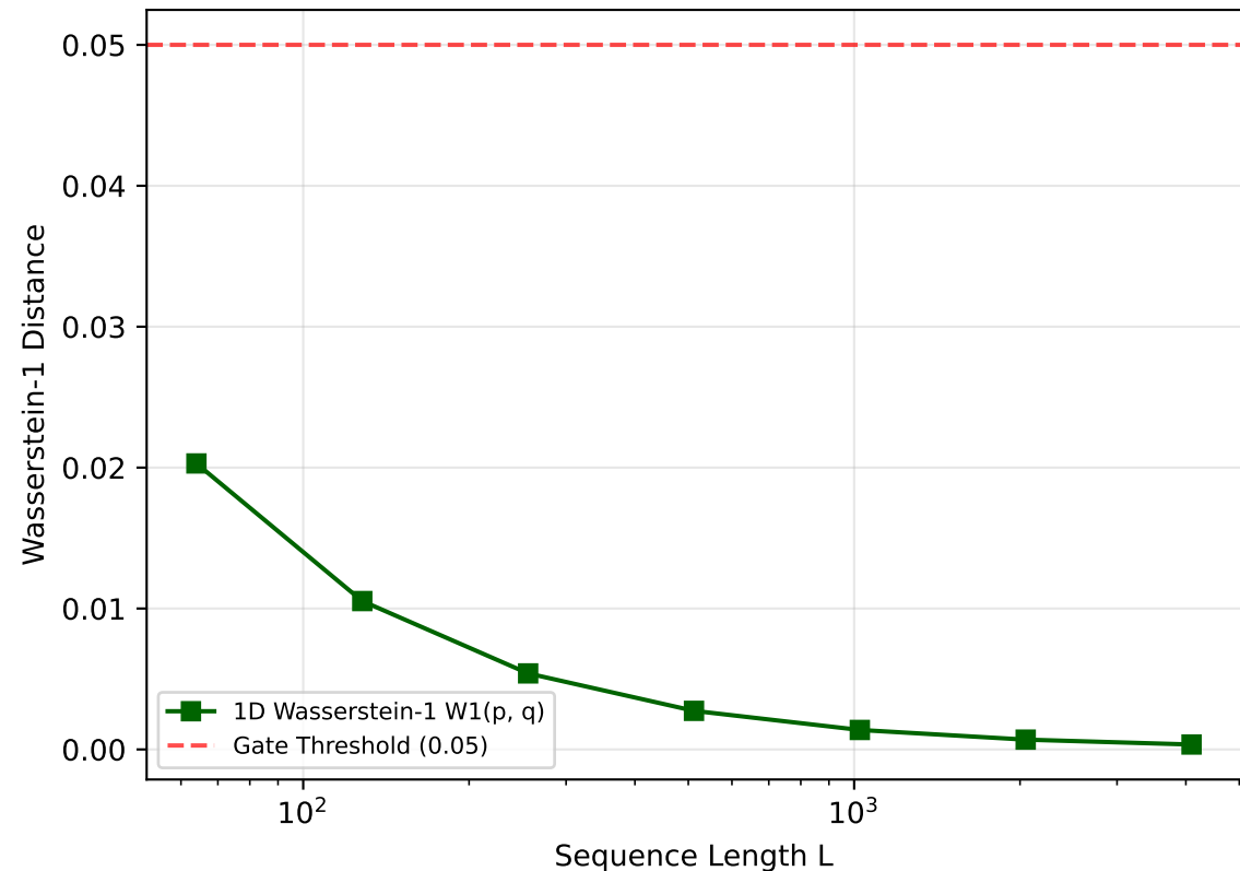
Attention Distribution Parity ( W1 \leq 0.05 )
