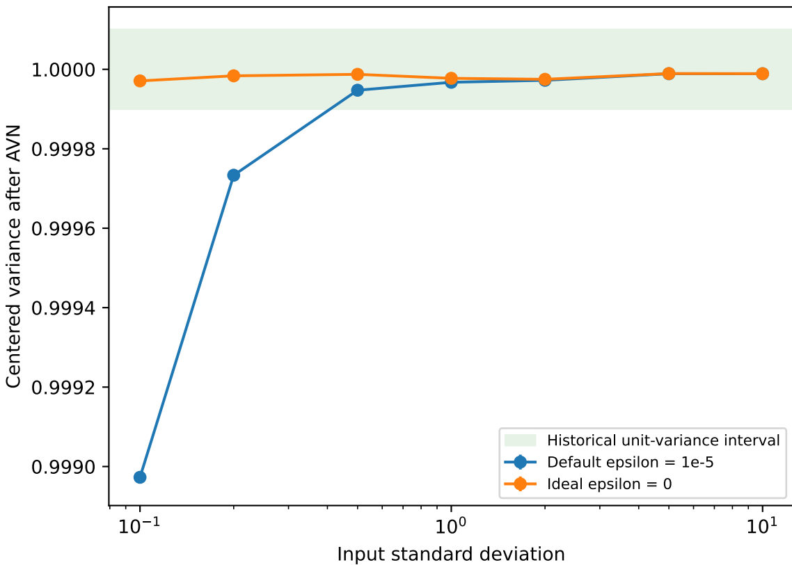
Phase 1 CPU study (fp64 moments, fp32 depth); 95% confidence intervals
