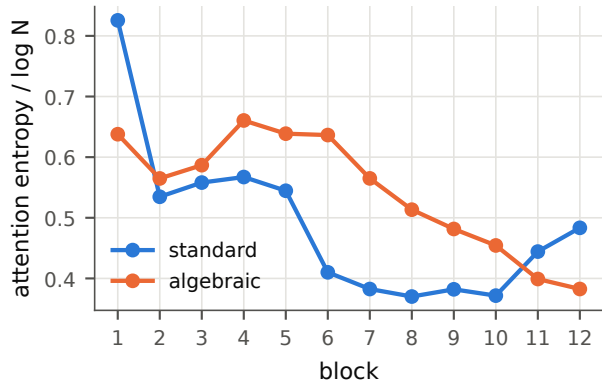
Attention entropy (trained ViT-B/16, seed 42)
