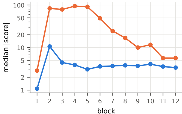
Score size
