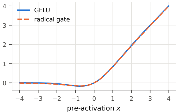
MLP gate
