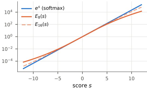
Attention kernel
