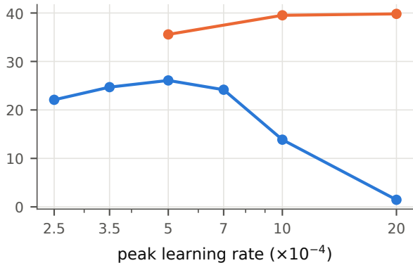
ViT-B/16, 224 px, 600M tokens
