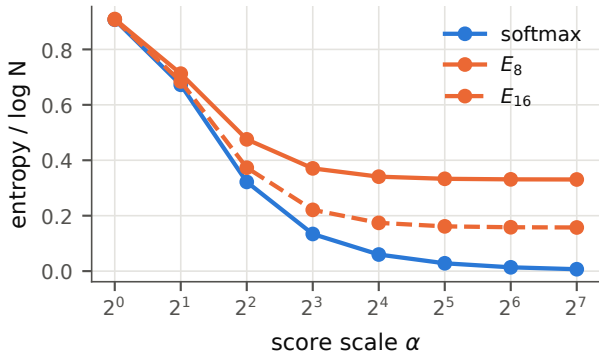
Attention entropy
