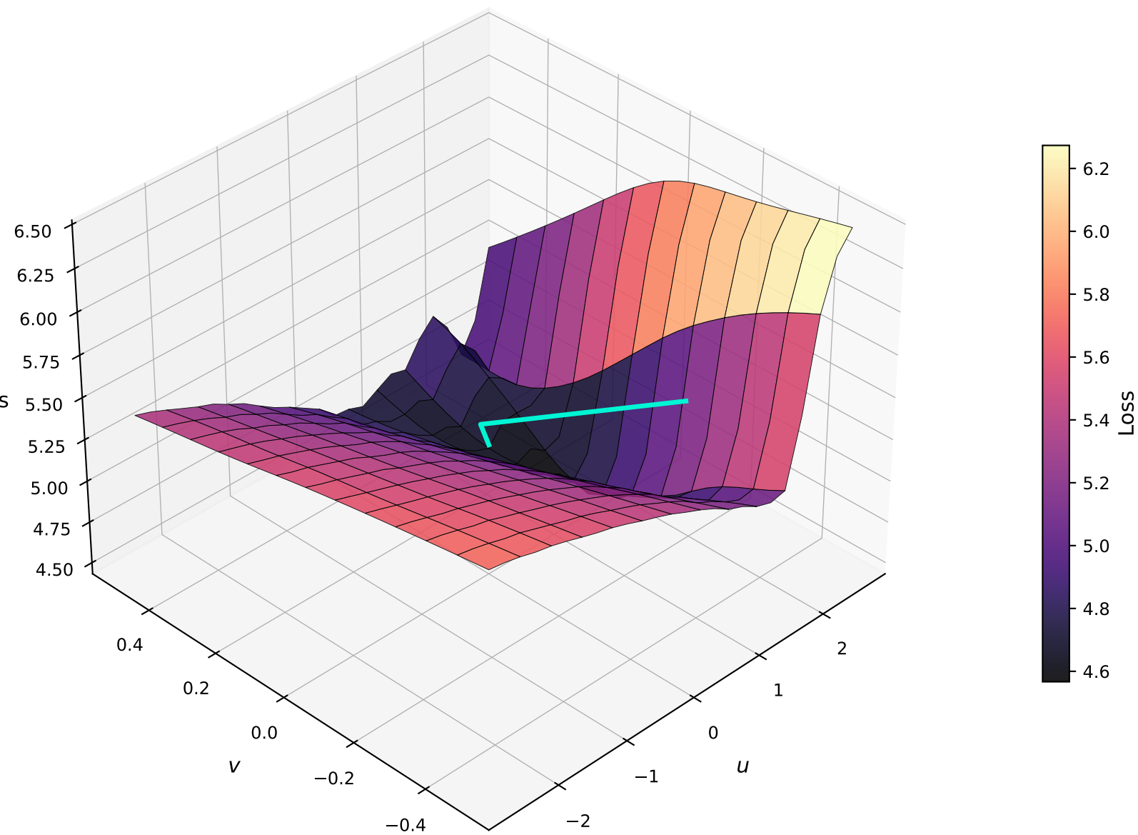
ATLAS 3D Reconstructed Loss Surface
