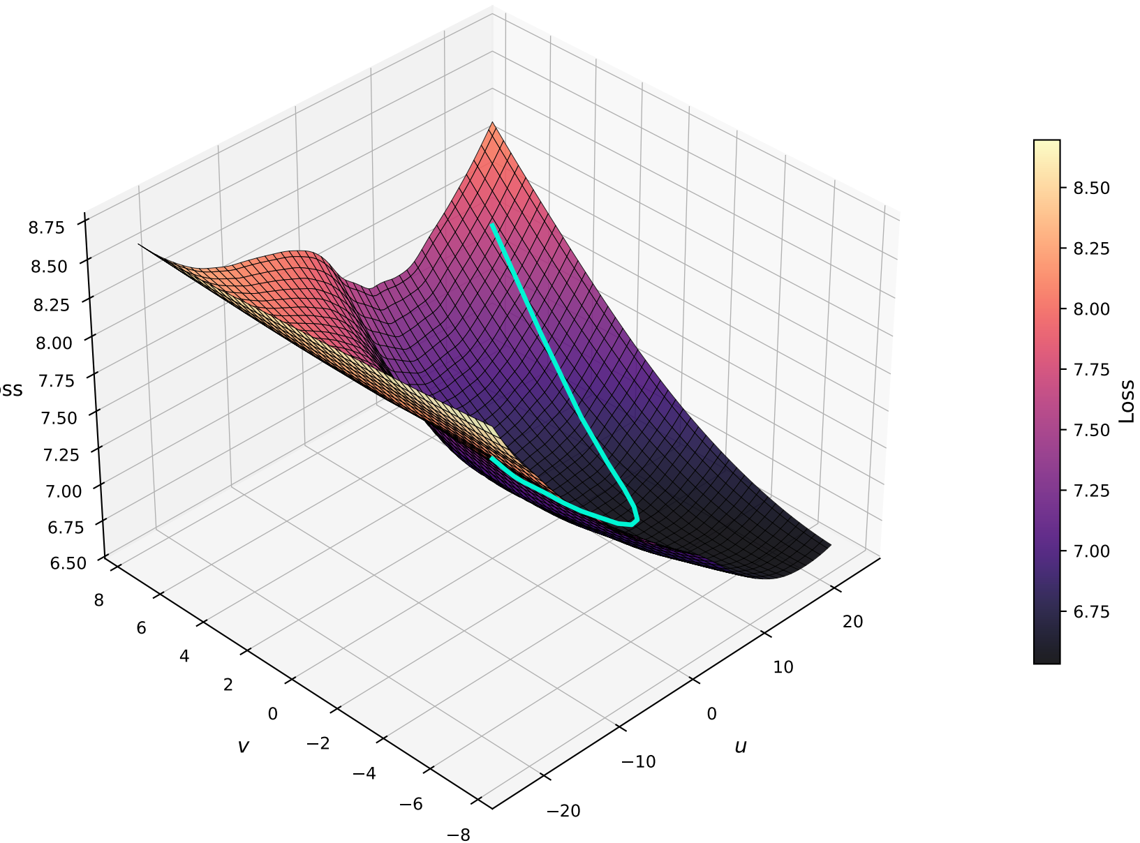
ATLAS 3D Reconstructed Basin: Causal Language Transformer on WikiText
