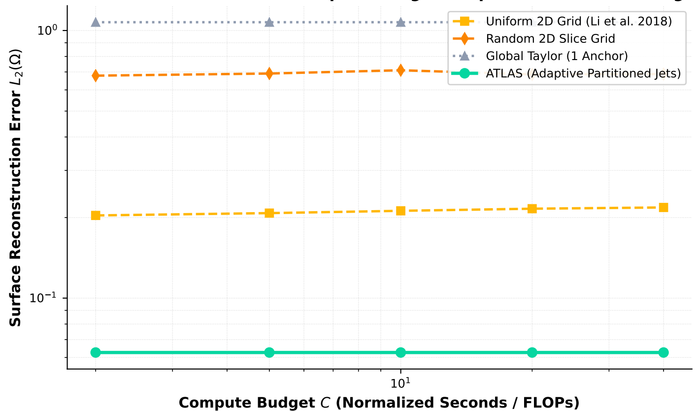
Reconstruction Error vs Compute Budget: Empirical Minimax Scaling
