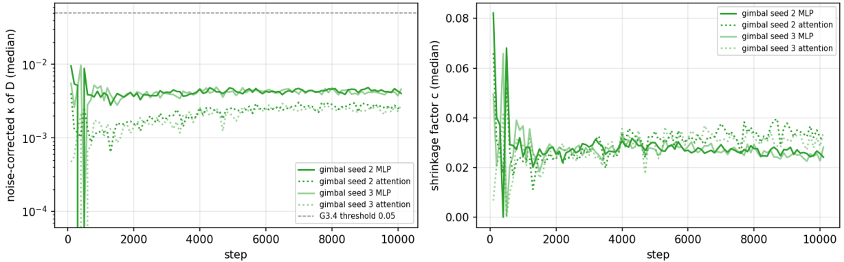
Figure 4: Gimbal’s runs: noise-corrected non-separability index of the flow’s variances (median over the matrices of each bucket; the predeclared premise threshold 0.05 dashed) and the empirical-Bayes shrinkage factor c .
