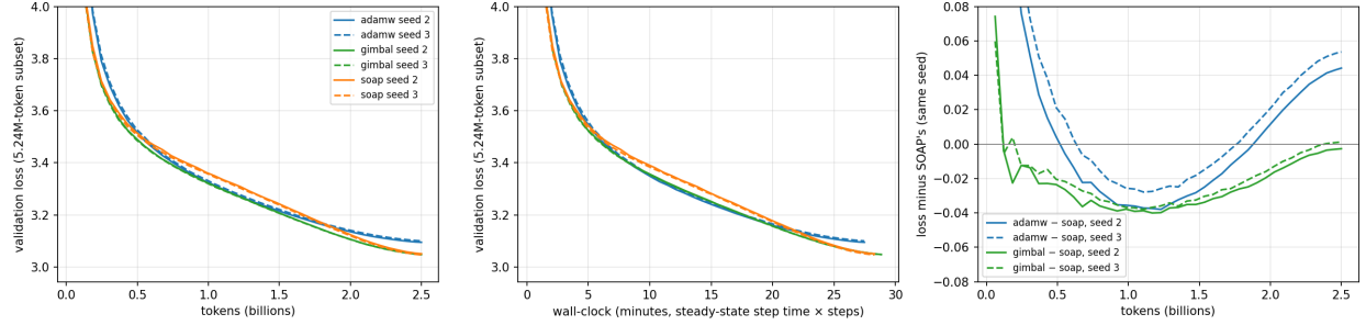
Figure 3: Validation loss on the 5.24M-token evaluation subset against tokens and against wall-clock (steady-state step time \times steps); solid seed 2, dashed seed 3.
