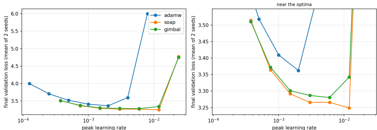
Figure 2: Tuning (614M tokens, mean of seeds 0 and 1): final validation loss against the peak learning rate, full range and near the optima (Gimbal with SOAP’s momentum, after the repair of appendix E).
