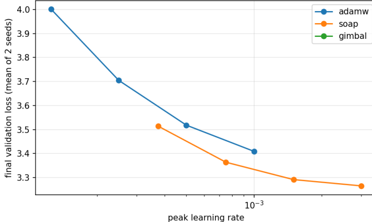
Figure 2: Tuning (614M tokens, mean of seeds 0 and 1): final validation loss against the peak learning rate (Gimbal with SOAP’s momentum, after the repair of appendix E).
