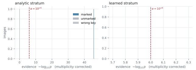
Figure 1: Marked, unmarked and wrong-key evidence for each stratum against the operating point. The wrong-key population sitting on top of the unmarked one is the statement that the detector reads a key, not an embedding.
