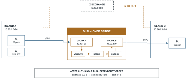
Fig. 3. Route-cut topology. Four application nodes span two isolated network segments joined by a shared exchange, which the experiment withdraws mid-run.
