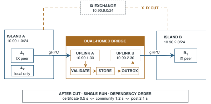
Fig. 3. Route-cut topology. Four application nodes span two isolated network segments joined by a shared exchange, which the experiment withdraws mid-run.
