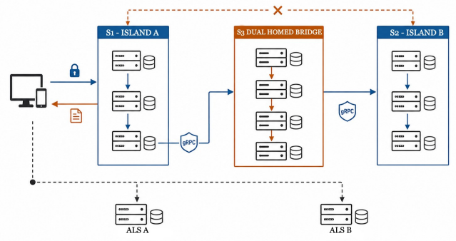
Fig. 1. System architecture: validating island nodes, a dual-homed bridge, and independent audit-log services.
