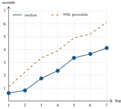
Fig. 4. Per-hop latency measured from in-transaction timestamps across the eight-node chain at a 1,000 ms drain interval. All the 200 envelopes reached hop 7.
