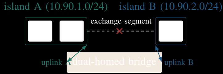
Fig. 2. Route-cut topology. Four application nodes span two isolated network segments joined by a shared exchange, which the experiment withdraws mid-run. The bridge is an application server, not an IP forwarder.
