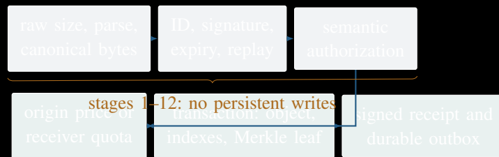
Fig. 1. Admission pipeline. State changes begin only after the cheap byte and validity checks have all succeeded.
