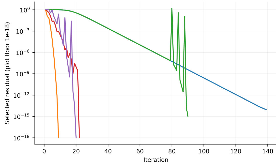
P11 — convergence by steps and by work
