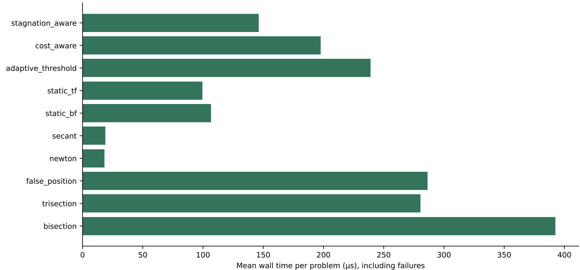
Paper benchmark — execution time
